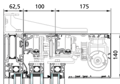
SL 45-T - thermally insulated (PST) With side panel and support profile
