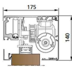
SL 45-S - leaf supplied by others Door leaf width 50 - 90 mm
