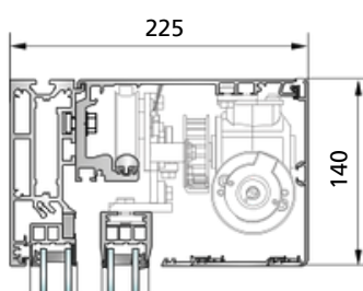
SL 45-S - standard (PSXP) With side panel and support profile
