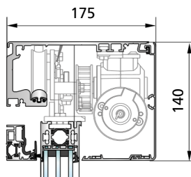
SL 45-S - leaf by others with connection profile Door leaf width 50 - 90 mm
