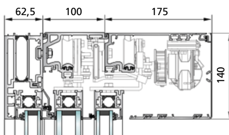
Standard - telescopic thermally insulated (PST) SL 35-T
