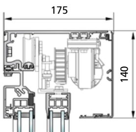
Standard - thermally insulated (PST) SL 35-S
