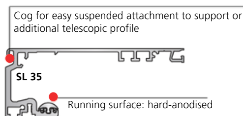
Compact - all glass (PSF) SL 35-C
