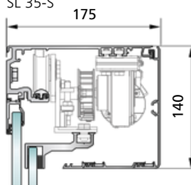
Standard - low-profile frame (PSA) SL 35-S
