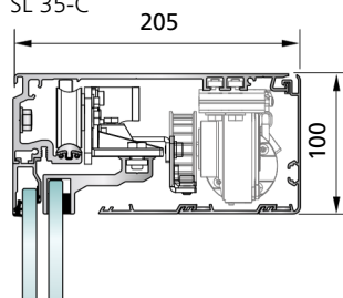
Compact - low-profile frame (PSA) SL 35-C
